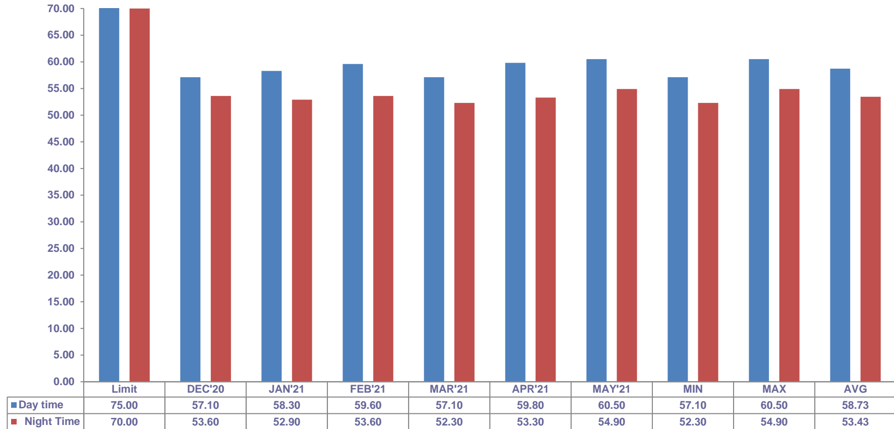
NOISE LEVELSAT HAULAGE ROAD ( DB ) AT LIME STONE MINE
